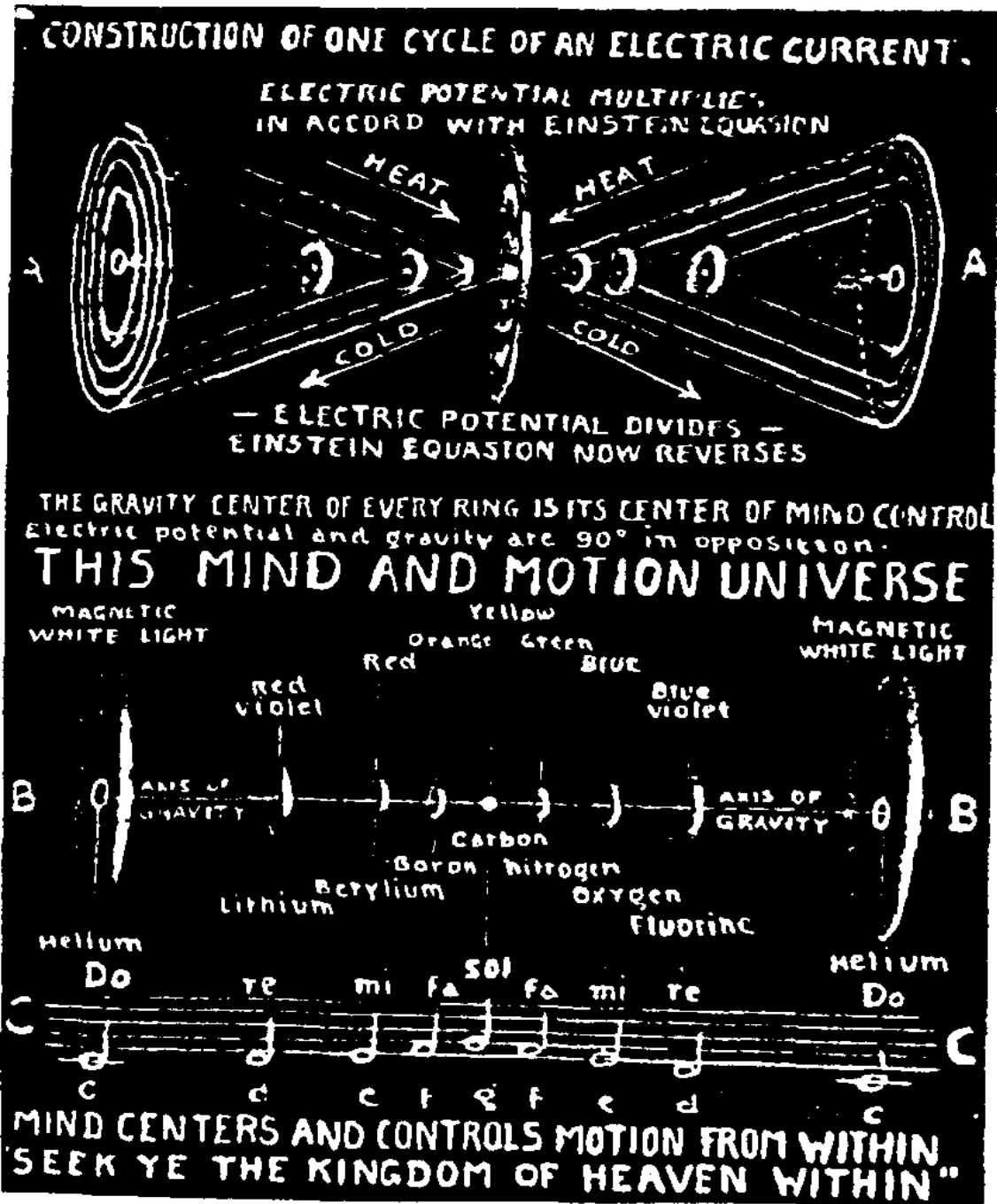
Fig. 42. Three examples of tonal rhythms of the electric current. Every cycle of an electric current is a complete octave of four pairs and an inert gas keynote. All motion in Nature is tonal and rhythmic. Its rhythms are geometrically and mathematically cube based.
