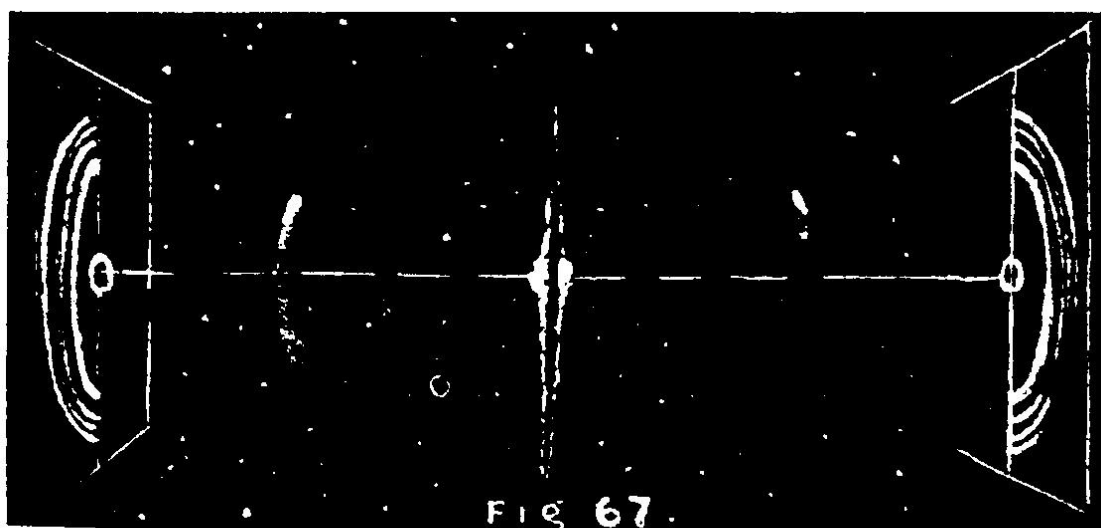
Fig 67. Illustrating principle of projection of Mind-desire energy into pairs of tones to create the nine octaves of tones, which constitute Nature. The spiral nebula—seen edgewise—which occupies the amplitude position in the wave current, corresponds with the loop of force which centers every polarized unit of an electric current.
