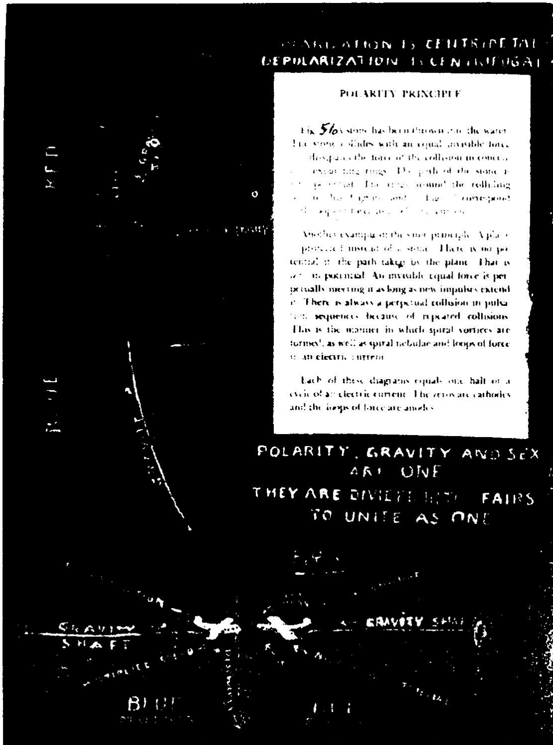
FIG 56 Every action in the universe is created in pairs. Its reaction is a part of it, and is simultaneously created. The union of every action with its reaction produces an effect which is always the image of the cause of the action.
