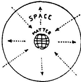
Fig. 22 Interchange between unequal opposites
