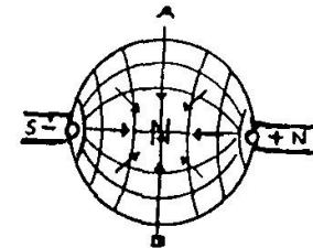
Fig. 27 Matter is formed between opposite poles in waves
