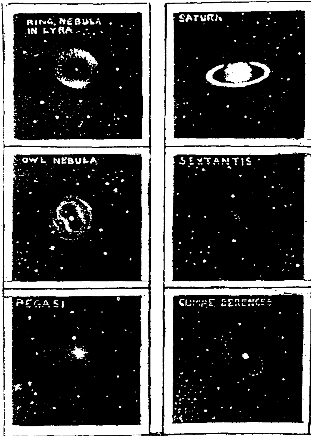
FIG. 52 The centering shaft, around which suns rotate, again compresses another sun into its vortex to repeat the process until all its mass disappears as rings. LYRA and Hydrae nebulae are good examples in the stellar system and Saturn well exemplifies how planets in our solar system, disappear into their zero.
