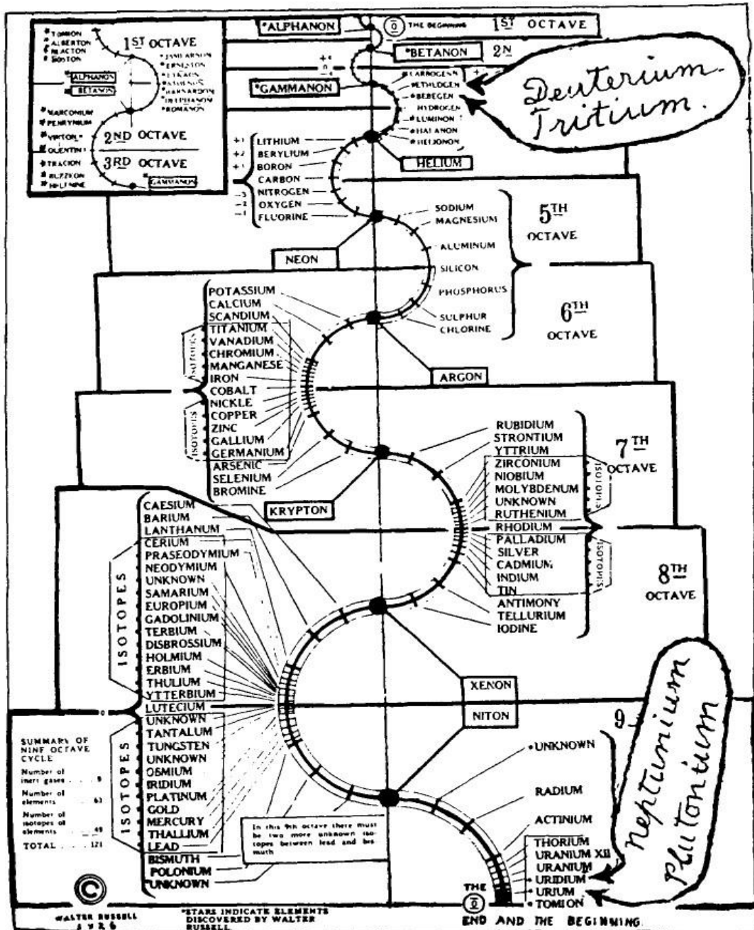
The Russell Periodic Chart of the Elements, No. 1
