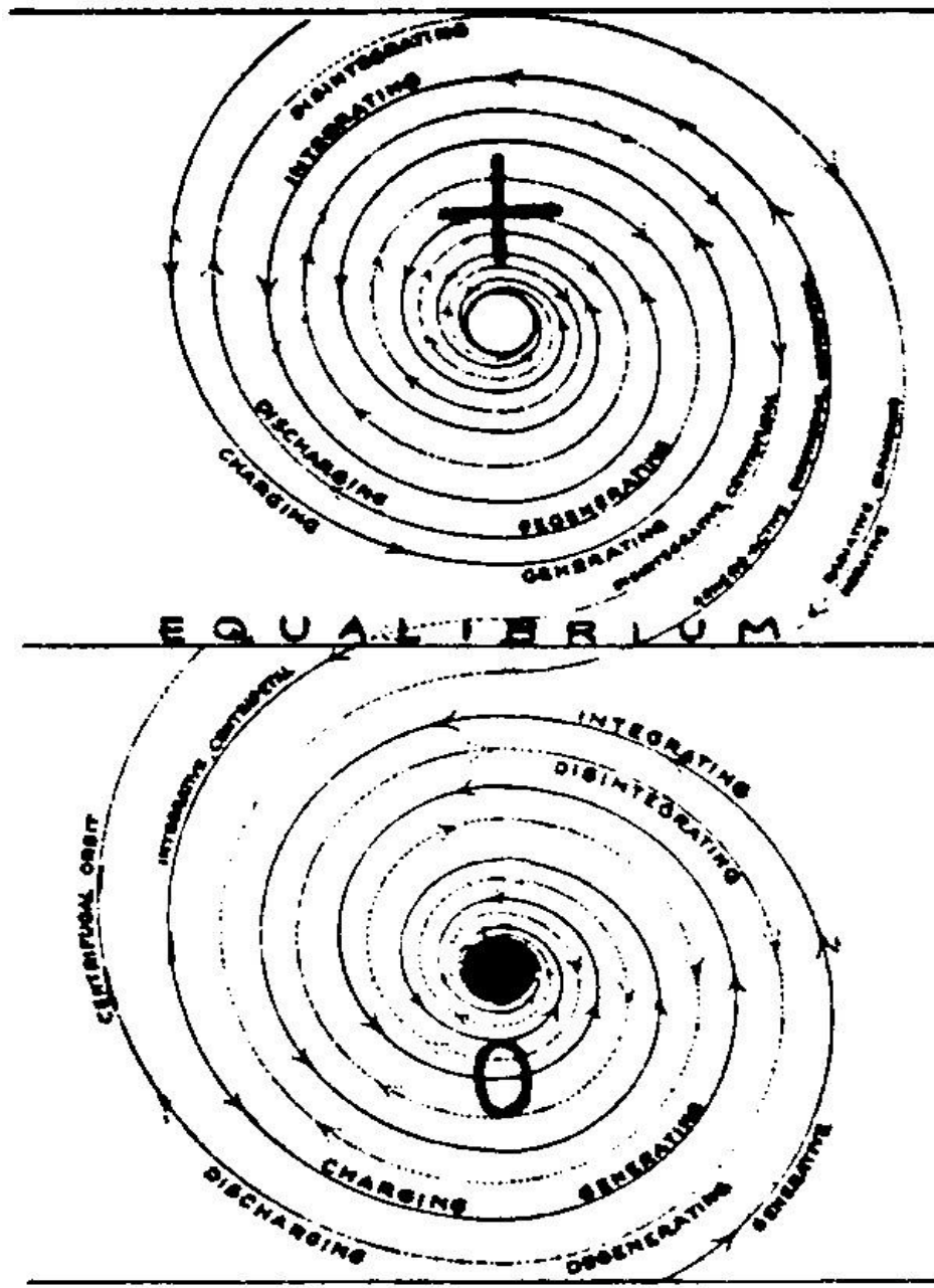
FIG. 66. Exemplifying the perpetual inter-relationship of matter and anti-matter as shown in Fig. 65, which gives and regives to each other for perpetual sequences of rebirths into each other. The outstanding characteristic feature of Nature is repetition. Life and death are other names for it. Reincarnation is still another name for it.
