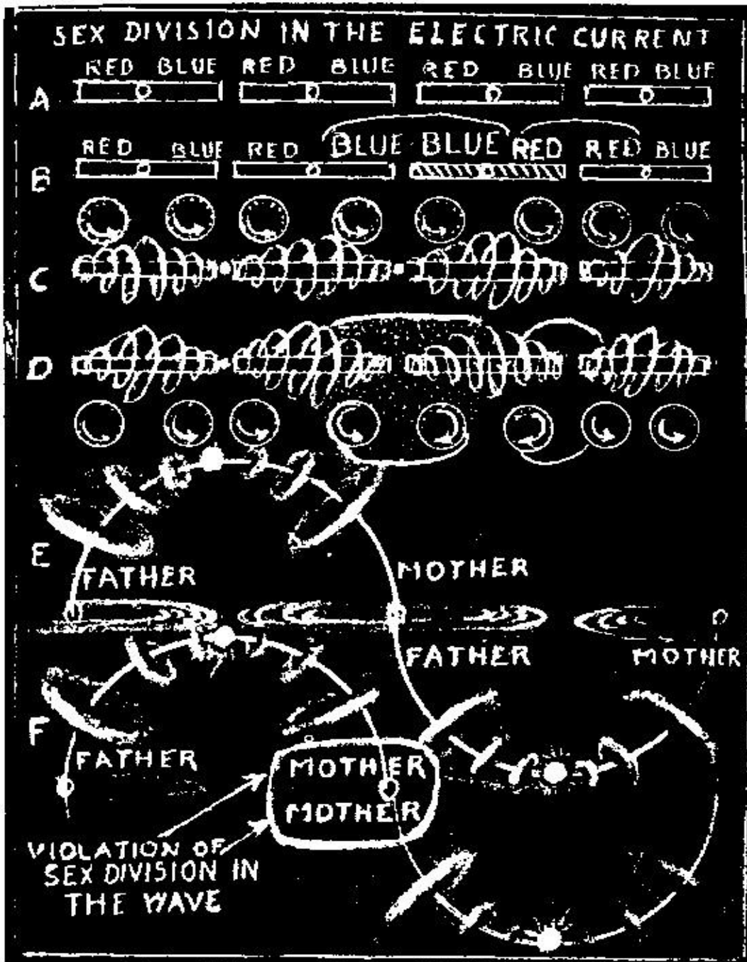
FIG. 17. Nature arranges her sex divisions in unit pairs in such a manner that opposite sexes can unite as one. Nature will not allow man to reverse this order by turning one unit of an electric current, or wave, around to make sex unity impossible.
